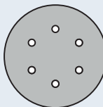
GLS 3 Ø 150 mm 6 holes Ø 10 mm on hole circle Ø 80 mm
