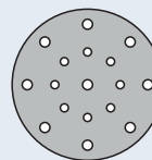
GLS 51 Ø 150 mm 8 holes Ø 10 mm on hole circle Ø 120 mm, 8 holes Ø 8 mm on hole circle Ø 65 mm + 1 centre hole Ø 10 mm
