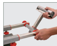
Angle adjustable end rollers
