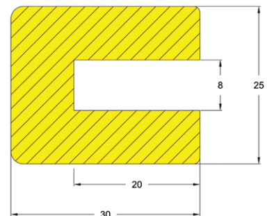
Rectangle 25/30/8
