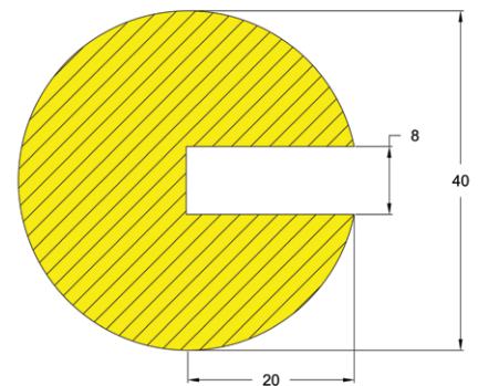
Semi Circular 40/40/8
