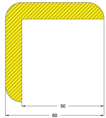
Right Angle 60/60
