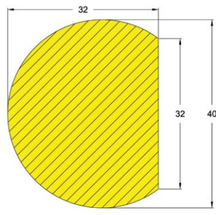
Semi-circular 40/32
