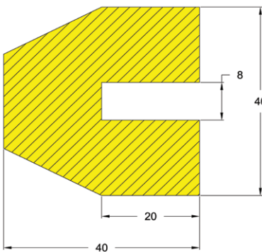
Trapeze 40/40/8
