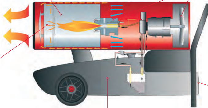
Burner Designed to ensure a perfect air-fuel mixture, resulting in an almost total combustion, with a CO 2 level of Oppm
