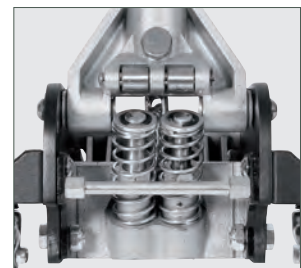
Dual pump system
