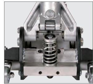
Single pump system
